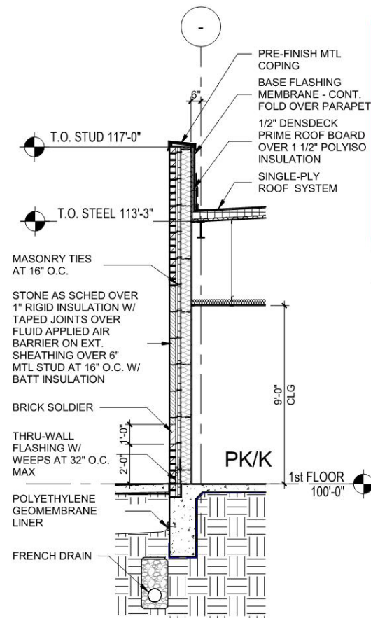
1 SECTION @ STONE SCALE: 1/4" = 1'-0"
