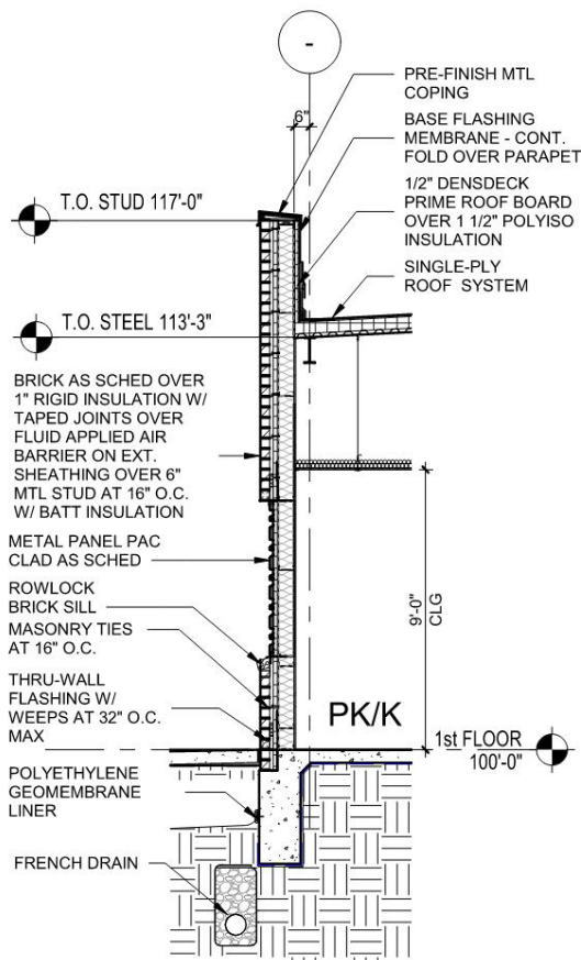
3 SECTION @ METAL PANEL SCALE: 1/4" = 1'-0"
