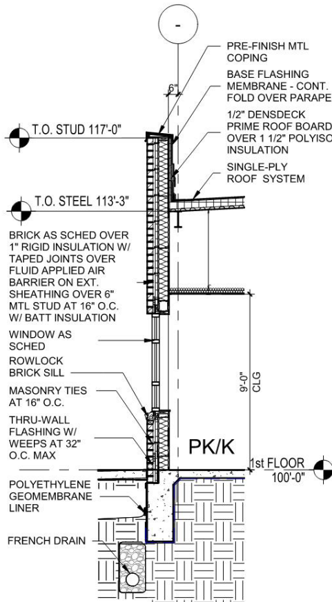
2 SECTION @ WINDOW SCALE: 1/4" = 1'-0"
